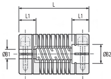
Coupling Type 703 6-Beam Non-Relieved
