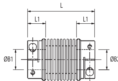
Coupling Type 538 & 539 Long (greater angular offsets or axial motion)
