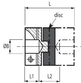
Coupling Type 234 & 235 Clamp style
