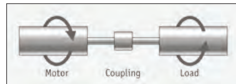
Fig. 11 Mode: Supply to motor discontinued, braking applied to load. Torque 'seen' by coupling = motor inertia - motor drag.
