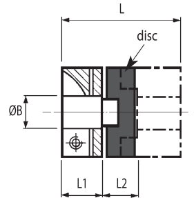
Coupling Type 452 or 453 Clamp style
