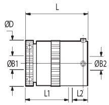
Rigid Coupling Type 281
