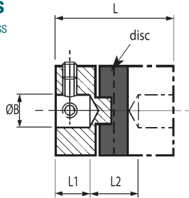
Coupling Type 232 Set Screw style
