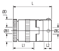
Oldham Coupling Type 285
